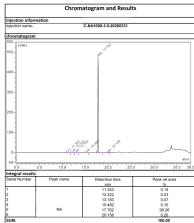
RP-HPLC - main peak RT 17.762 min (99.26%) - reproduced from source lab report
